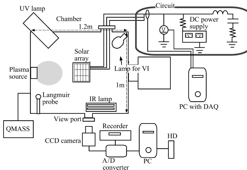
Fig. 3 Experimental system.
